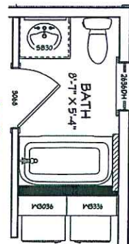
1st Floor
